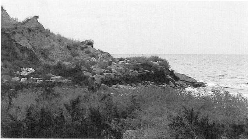
Fig. 6: The Kamennyi cape in November, 2012.
