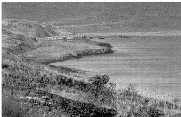
Fig. 3: September, 2011. The sea bottom that emerged above water after the Taman event.
