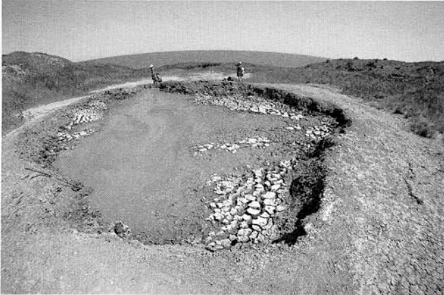
Fig. 10: “Azovskoe Peklo” mud volcano state is on reduced activity.
